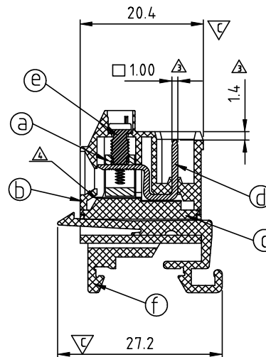
SECTION P-P
