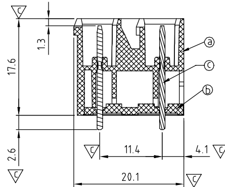
SECTION P-P
