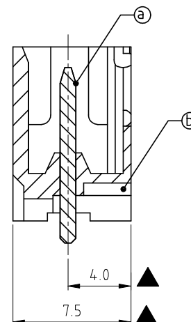
SECTION P-P
