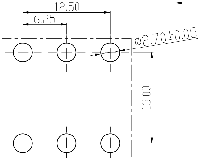
PCB LAYOUT
