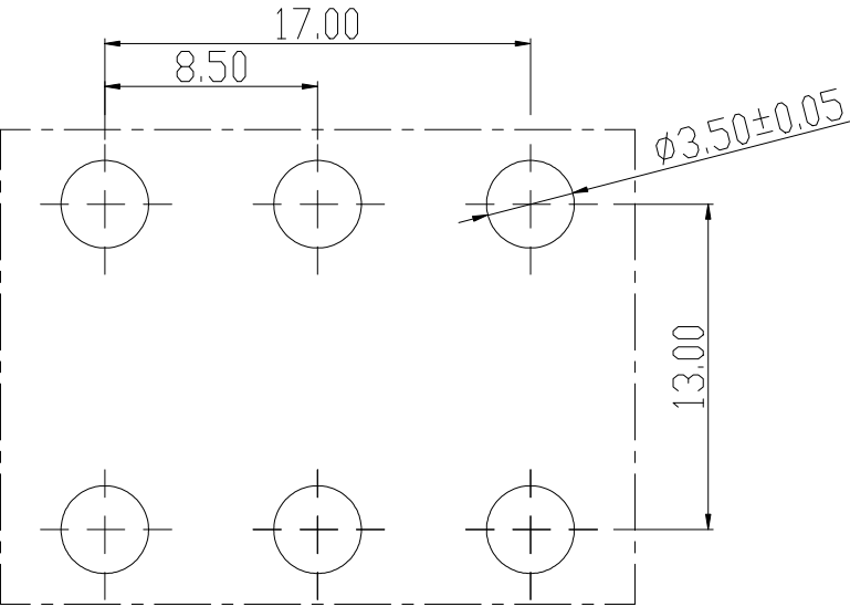
PCB LAYOUT
