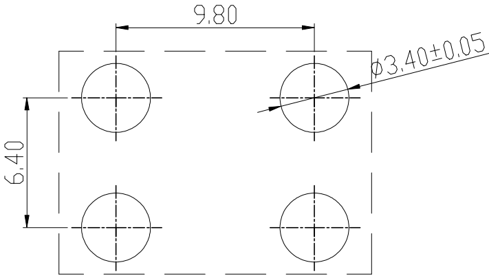
PCB LAYOUT
