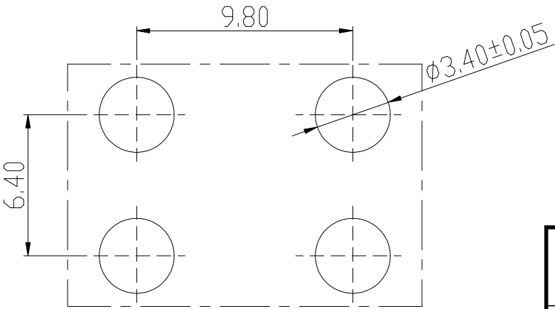
PCB LAYOUT
