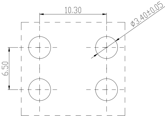
PCB Layout
