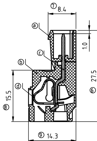
SECTION E-E
