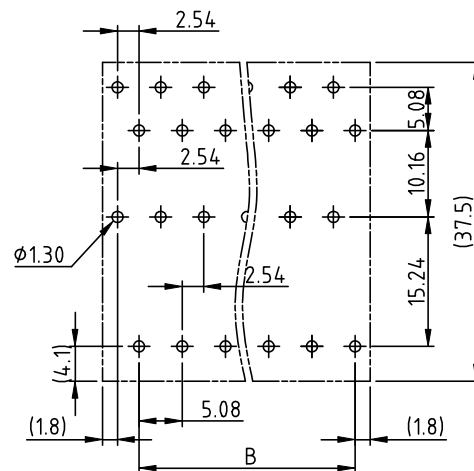
PCB Layout
