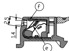
Section P-P
